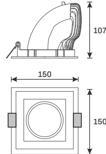
Cut-Out: 140 x 140mm *All dimensions are in mm.
